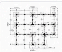
FOOTING LAYOUT PLAN
