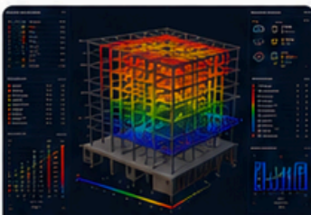
STRUCTURAL ANALYSIS
